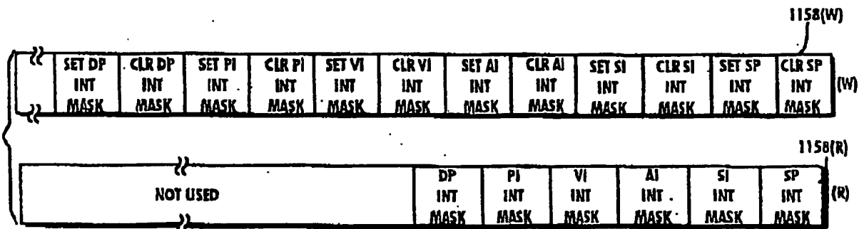
Fig. 39D INT MASK REGISTER
